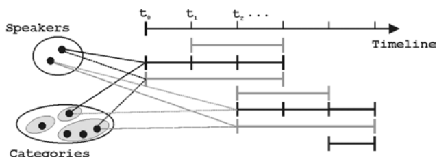
Figure 2: “Single timeline, multiple tiers” data model
